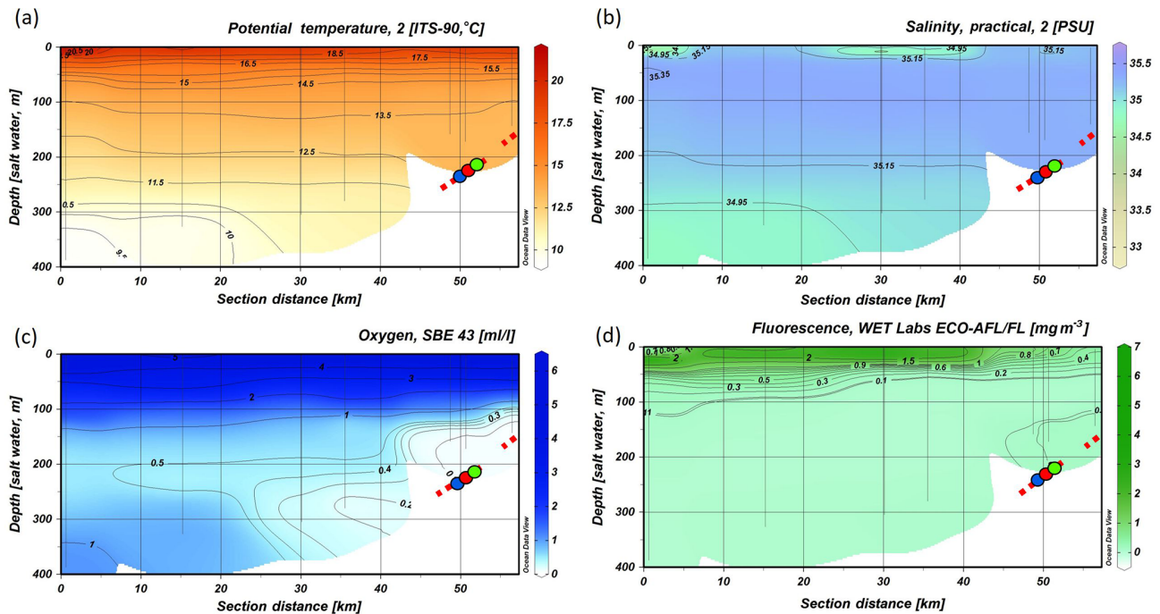
Figure 4. CTD transect across the Namibian margin (see Fig. 1b for location). Data are presented for (a) potential temperature (°C), (b) salinity (PSU), (c) dissolved oxygen concentrations ( \text{mL L}^{-1} ), note the pronounced oxygen minimum zone (OMZ) between 100 and 335 m water depth, and (d) fluorescence ( \text{mg m}^{-3} ) (data plotted using Ocean Data View v.4.7.8; http://odv.awi.de , last access: 12 February 2016; Schlitzer, 2011). The occurrence of fossil CWC mounds is indicated by a red dashed line, colored dots indicate bottom lander deployments.
