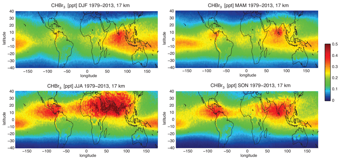
Figure S2: Modelled seasonal mean distribution of \text{CHBr}_3 at 17 km for DJF (December-February), MAM (March-May), JJA (June-August), and SON (September-November) 1979-2013.
