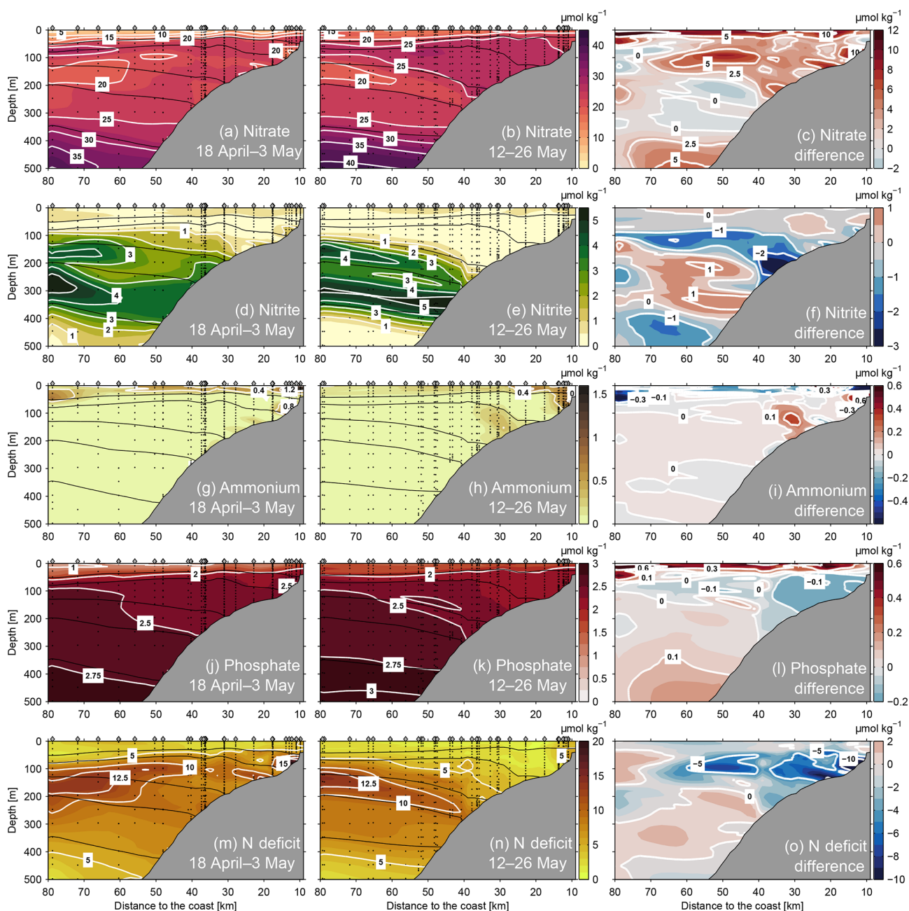
Figure 11. Nitrate (top row), nitrite (second row), ammonium (third row), phosphate (fourth row) concentrations and nitrogen deficit (bottom row) at 12° S during 18 April–3 May 2017 (left panels) and 12–26 May 2017 (middle panels). Concentration difference of the respective parameters between the two time periods are shown in the right panels. Black lines indicate the distribution of isopycnals ( \sigma_\theta ) at 25.6, 25.9, 26.2, 26.4 and 26.7 \text{kg m}^{-3} . Grey diamonds mark the positions of CTD stations and black circles mark the position of bottle samples in the water column.
