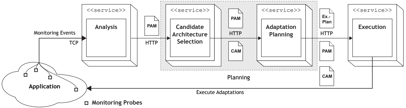
Figure 1: iObserve Architecture - Each MAPE-K phase is represented by an independent service
