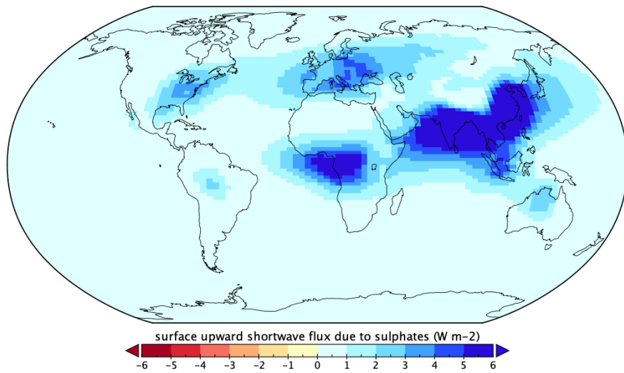
Figure S1: Clear-sky effective radiative forcing (ERF) from sulphate aerosols in the UVic ESCM 2.10. The global mean ERF amounts to 0.99 W m^{-2} , for comparison Stevens et al., 2017 have a global mean clear sky ERF of 0.67 W m^{-2} .
