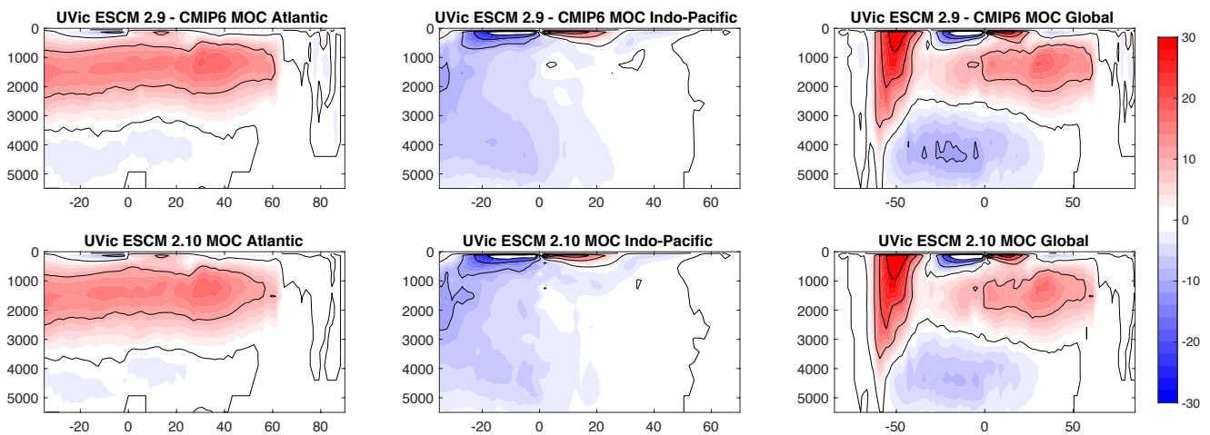
Figure S4: Ocean section of meridional overturning in units of Sv for the Atlantic Ocean including the Arctic Ocean (left column), the Indo-Pacific Ocean (middle column), and the global average (right column). From top to bottom are shown the published UVic ESCM version 2.9 by (Eby et al., 2013) spun-up and forced with CMIP6 forcing, and the UVic ESCM version 2.10, both as a mean of the 1980-2010 period.
