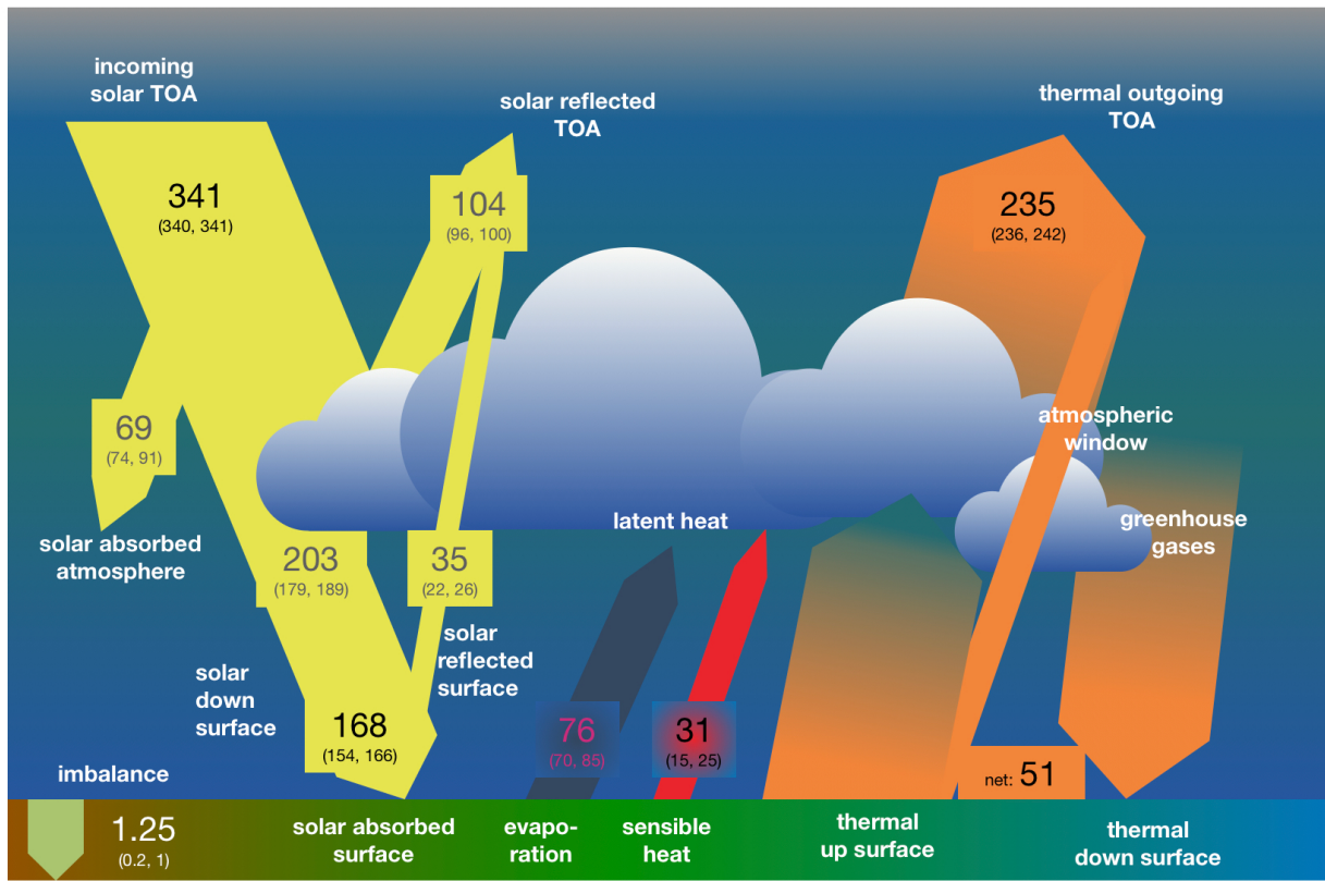
Figure S5: Schematic diagram of the global mean energy balance of the UVic ESCM 2.10 adapted from Wild et al., 2013. Magnitudes of the globally averaged energy balance components, black numbers indicate estimates directly taken from the model output, grey numbers have been derived by calculations given albedo values from the model, and the latent heat was calculated using the evaporation estimates from the model assuming a conversion factor of 2,260 kJ/kg. Uncertainty ranges are taken from (Wild et al., 2013), representing present day climate conditions at the beginning of the 21th century. Units Wm^{-2} .
