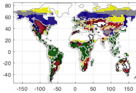
Figure S7: Map of predominant plant functional types in the UVic ESCM 2.10 for the period of 1980-2010, color indicate broadleaf tree (green), needleleaf tree (blue), C3 and C4 grasses (yellow), crops (red) and shrubs (grey).
