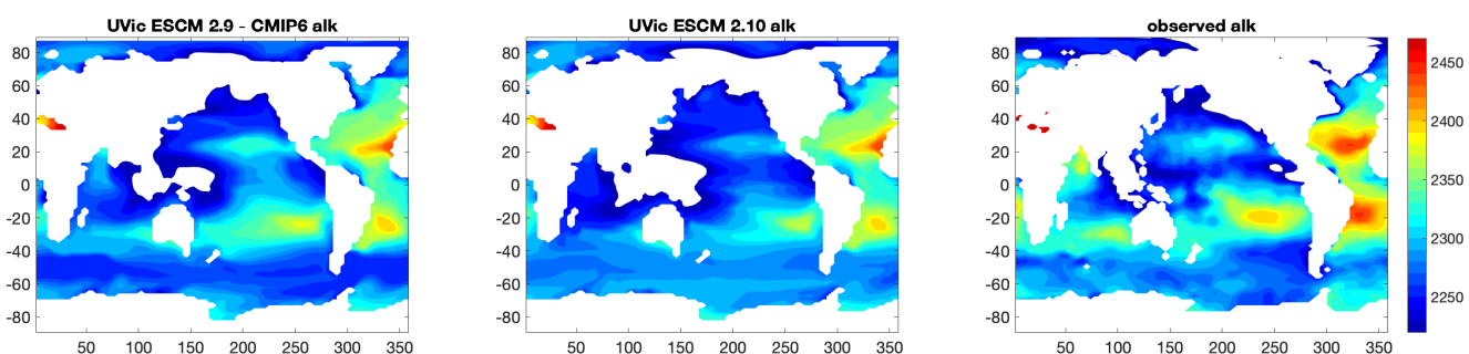
Figure S18: Maps of sea surface alkalinity in units of \mu\text{mol kg}^{-1} for the published UVic ESCM version 2.9-02 (Eby et al., 2013) spun-up and forced with CMIP6 forcing, for the UVic ESCM 2.10, and for the Global Ocean Data Analysis Project (GLODAP) mapped climatologies version 2 (Lauvset et al., 2016).
