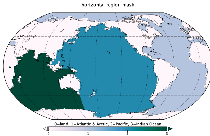
Figure S8: Map showing the partitioning of the UVic ESCM into different ocean basins.
