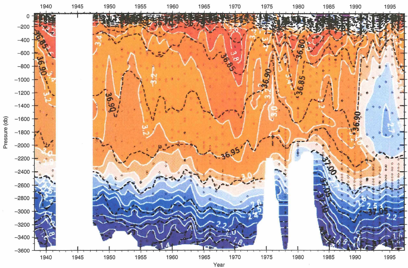
Figure 11 Demonstration of interannual variability (1938-97) of potential temperature in °C (colors and white isotherms) and potential density \delta_{1.5} ( \text{kg m}^{-3} (dashed black lines) referenced to 1500 dbar pressure level. (After I Yashayaev et al. , www.mar.dfo-mpo.gc.ca/science/ocean/woce/absea/labsea_poster.html .)
