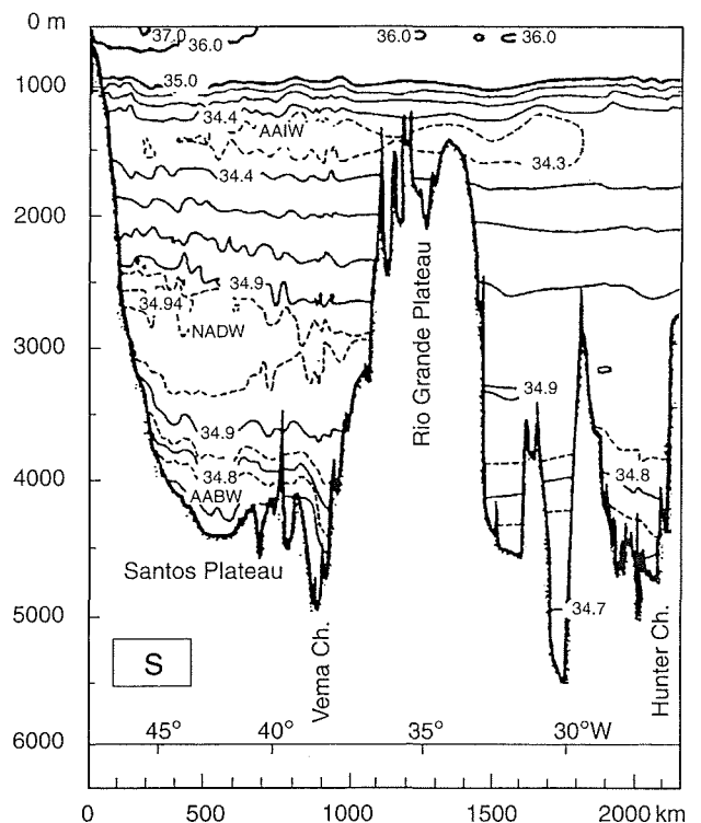
Figure 14 Salinity distribution (PSU) on a section across the Rio Grande Rise, South Atlantic, at nominally 30°S between the slope off Brazil and the Middle Atlantic Ridge. The Vema and Hunter Channels allow an active equatorward flux of Antarctic Bottom Water (AABW). More saline North Atlantic Deep Water (NADW) is advected poleward above the bottom water. On top of the abyssal layers lower saline Antarctic Intermediate Water (AAIW) again spreads equatorward. (Reproduced with permission of the American Meteorological Society from Hogg et al. , 1999.)
