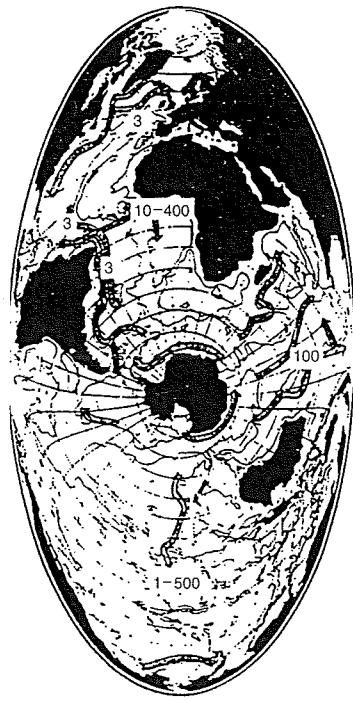
Figure 5 Some estimates of cross-isotherm diffusivity in \text{cm}^2\text{s}^{-1} in the abyss of the world's oceans. (After Hogg, 2001, © Academic Press.)
