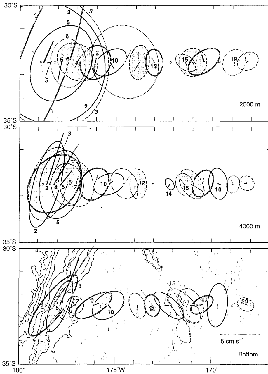
Figure 18 Long-term observations of the deep western boundary current system at 32°30'S at three instrumented abyssal layers (2500, 4000m, near-bottom) of the Pacific. Mooring locations at dots are shown by the origin of the presented mean velocity vectors. Ellipses inform about the current's stability in form of the root mean square amplitudes. Small italics in the lower panel indicate depths in km. Bolder numbers are mooring identifiers. Note the clear bottom-intensified flow of Antarctic Bottom Water. The returning North Pacific Deep Water flow is less confined and highly variable. (Reprinted from Progress in Oceanography 43, Whitworth et al. , on the deep western-boundary current in the Southwest Pacific Basin, 1-54 © (1999) Elsevier Science and the American Meteorological Society.)
