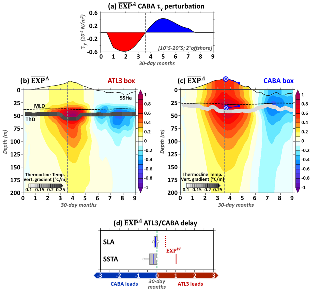
Figure 11. Interannual variability simulated in \overline{\text{EXP}}^A , in which there are coastal wind-stress fluctuations off Southwest Africa (cf. Table 1). (a) Timeseries of meridional wind-stress perturbations ( 10^{-2} \text{ N}\cdot\text{m}^{-2} ) averaged in the CABA box. (b) Same as Figure 7a for \overline{\text{EXP}}^A . (c) Same as Figure 7b for \overline{\text{EXP}}^A . Circled-crosses position the CABA maximum surface and subsurface temperature anomalies. Round arrows recall \overline{\text{EXP}}^W maximum surface and subsurface temperature anomalies from Figure 7b. (d) Same as Figure 6 for \overline{\text{EXP}}^A , using plain blue line for the mean of the 10 ensemble member lag estimates. Red vertical lines recall the mean of the 10 ensemble member lag estimates of \overline{\text{EXP}}^W .
