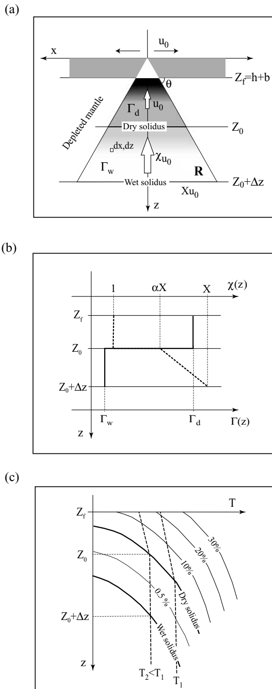
Figure 9. (a) Sketch summarizing the melting process for mantle corner flow beneath spreading ridges. U_0 is the spreading rate and \chi is the mantle upwelling ratio. In our model, \chi = 1 , passive upwelling, above the dry solidus. The final depth of melting is Z_f , which is determined by the lithospheric lid (old lithosphere, b , and newly formed oceanic crust, h ). The initial depth of melting is Z_0 , which is defined by the intersection of the dry solidus and the mantle adiabat. \Delta Z is the thickness of the damp melting area. R is the section of the melting region for mantle corner flow, dx, dy indicate an element of mantle. (b) Diagram indicating the values of the upwelling ratio at the base of the melting zone, X , the slope of the upwelling ratio decay within the damp melting zone, \alpha , and the melt productivity within the dry, \Gamma_d , and damp, \Gamma_w , melting regions in our melting model (see details in Sections 6.1 and 6.2). The thick solid line represents the melt productivity, \Gamma(z) , and the thick dashed line the upwelling ratio, \chi(z) . (c) Scheme of a phase diagram illustrating the dry and wet solidus (thick solid lines), the mantle adiabat for different potential temperatures (dashed lines), and the melting rates for given \Gamma_d and \Gamma_w (thin solid lines).
