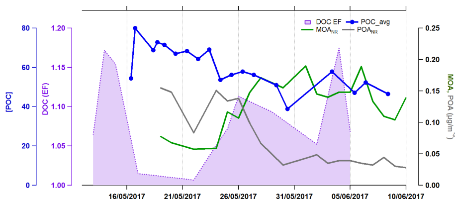
Figure 7. Time series of the DOC enrichment factor (EF), POC concentrations, and PMF organic factors \text{MOA}_{\text{NR}} and \text{POA}_{\text{NR}} .
