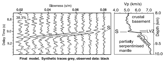
Figure 3. Comparison of synthetic results with original traces around S. The match is very good for S – a misfit of 38.3% in a 350 ms window about S results. Right: Final velocity model (black) overlain on initial Vp model (gray), showing fine structure revealed by the inversion. Note the presence of a 50 m. low velocity zone (LVZ) immediately above S and a gradient zone below S. S itself is resolved as a sharp step increase in velocity, not present in the starting model.
