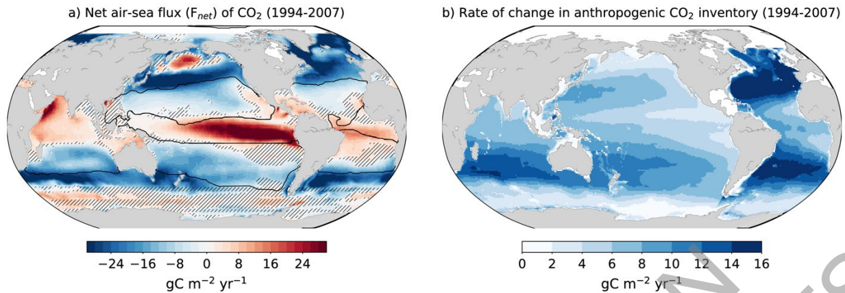
Figure 5.9: Comparative regional characteristics of the mean decadal (1994–2007) sea-air \text{CO}_2 flux ( F_{net} ) and ocean storage of anthropogenic \text{CO}_2 . (a) regional sink–source characteristics for contemporary ocean air-sea \text{CO}_2 fluxes ( F_{net} ) derived from the ensemble of 6 observation-based products using SOCATv6 observational data set (Bakker et al., 2020; Landschützer et al., 2014; Rödenbeck et al., 2014; Zeng et al., 2014; Denvil-Sommer et al., 2019; Gregor et al., 2019; Iida et al., 2020) Warm colours depict outgassing fluxes and black contours characterise the super-biomes defined from Fay and McKinley (2014) and adjusted by Gregor et al., (2019) also used to calculate the variability in regional flux anomalies (Supplementary Materials Figure 5.SM.1); and (b) the regional characteristics of the storage fluxes of \text{CO}_2 in the ocean interior for the same period (Gruber et al., 2019a). The dots reflect ocean areas where the 1-sigma standard deviation of F_{net} from the 6 observation product is larger than the magnitude of the mean. This reflects source-sink transition areas where the mean F_{net} is small and more strongly influenced by spatial and temporal variability across the products. Further details on data sources and processing are available in the chapter data table (Table 5.SM.6).
