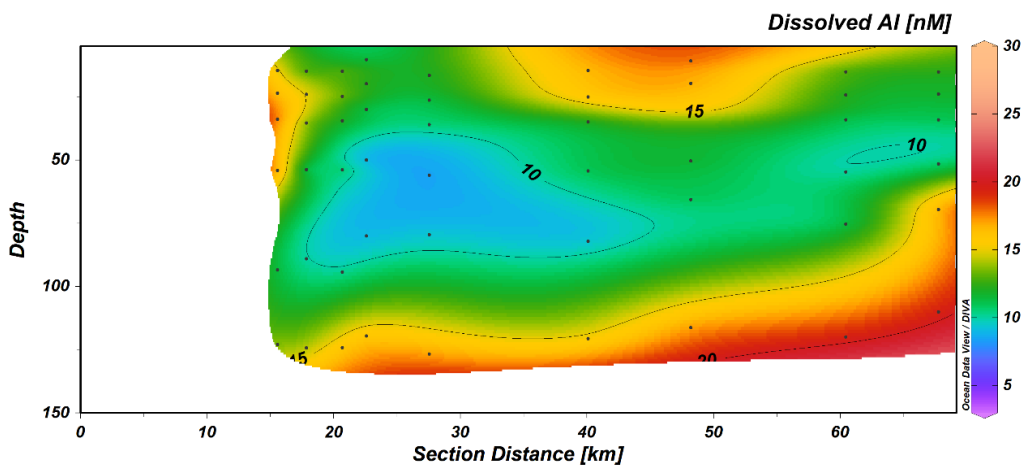
Fig. 5.9 Vertical profiles of dissolved Al concentrations in the surface ocean above the Rainbow hydrothermal vent and up to >60 km distance.
