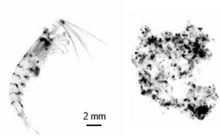
Fig. 5.26 Example of plankton (left) and marine snow (right) images taken with the UVP5 during SO288.
