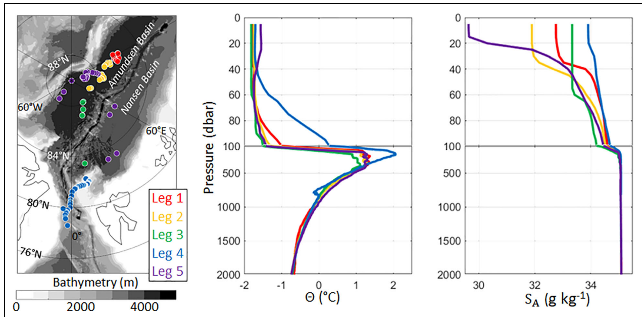
Figure 8. Hydrographic properties during the five legs. Left: location of all of the full-depth casts with the Polarstern-hydroholog-CTD during the Multidisciplinary drifting Observatory for the Study of the Arctic Climate drift, color-coded per leg; bathymetry from GEBCO (Weatherall et al., 2020). Right: for each leg, corresponding CTD profiles of conservative temperature ( \Theta ) and absolute salinity ( S_A ), median-averaged in time for each leg and vertically averaged into 5-dbar bins (1 dbar 1 m). CTD data are preliminary and available in Tippenhauer et al. (2021). Number of casts, distance, and time period differ for each leg (see Figure 7 ). CTD = conductivity-temperature profiling through depth. DOI: https://doi.org/10.1525/elementa.2021.00062.f8
