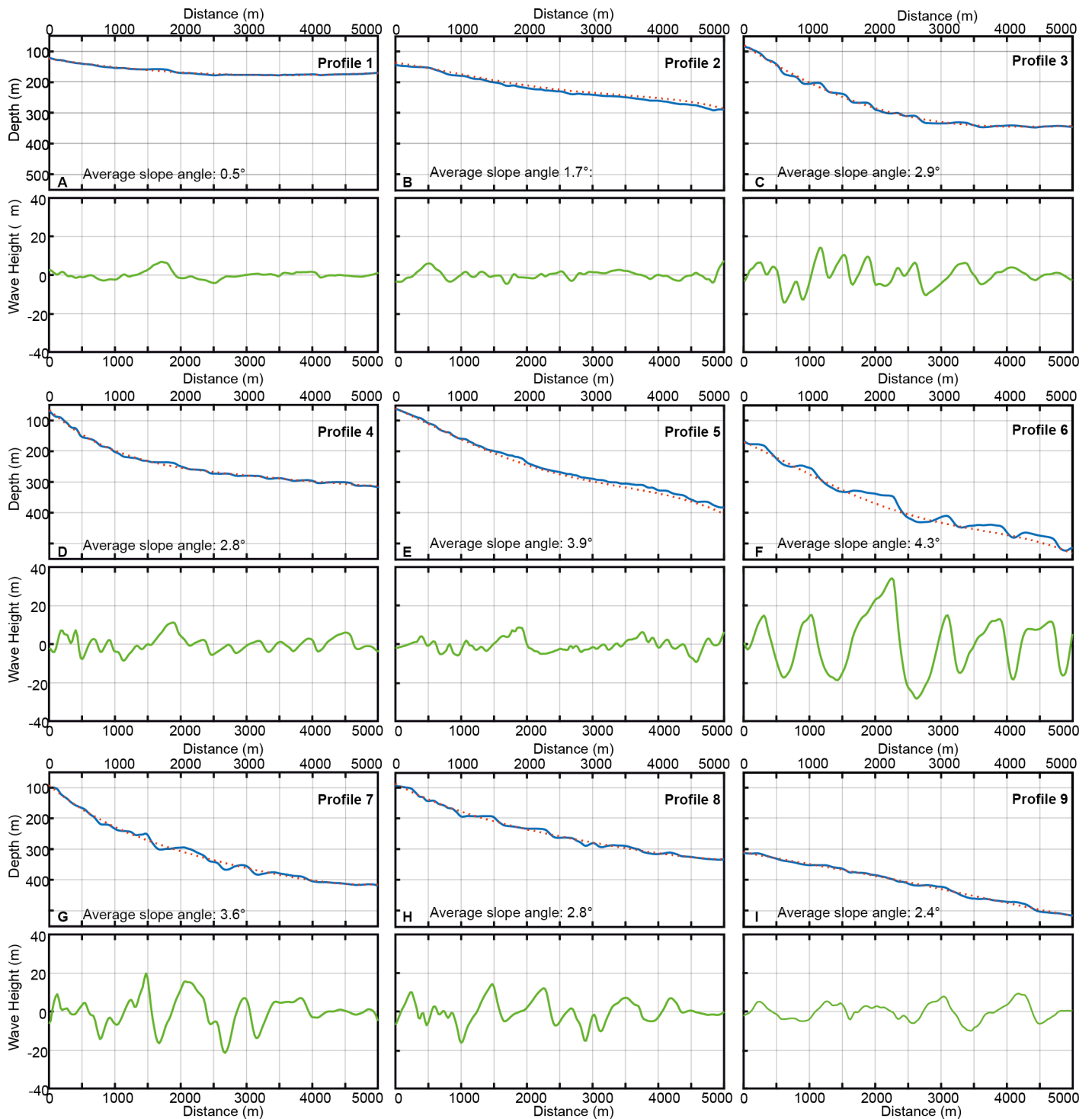
Figure S1: (A) – (I) Morphological profiles of Santorini's flanks (blue line), regression curves through these profiles (dotted red line), and difference of both (green line) showing the wavelength and wave height of USBs.).
