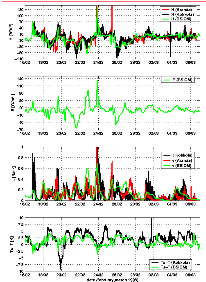
Figure 4. Time series of sensible heat flux H , latent heat flux E , momentum flux \tau and surface-air temperature difference T_s-T at Kokkola and RV Aranda in comparison with model data at Kokkola.
