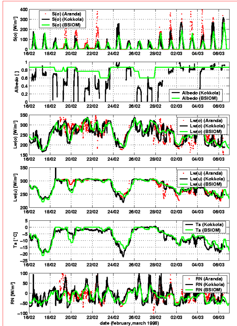
Figure 3. Time series of radiation parameters downwelling short-wave radiation S(o) , albedo, downwelling long-wave radiation Lw(o) , upwelling long-wave radiation Lw(u) , surface temperature T_s and net radiation RN at Kokkola and RV Aranda in comparison with model data at Kokkola.
