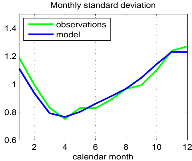
Figure 2.18: Seasonal dependence of standard deviation of Niño3 SST in observations (1950-2002) compared to the results of the seasonal dependent recharge oscillator model with constant stochastic excitation.
