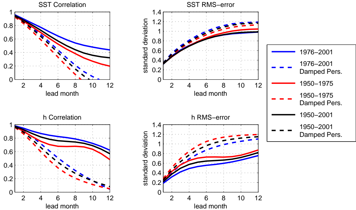
Figure 2.5: Forecast skill of the recharge oscillator model for Niño3 SSTA (top) and equatorial Pacific thermocline depth anomalies (bottom). The coloured lines show cross-validated forecast skills. The time intervals given in the legend refer to the period used for the forecast skill evaluation, while in each case the other interval was used to fit the parameters. For the black lines the whole time period was used for the parameter fit and for the evaluation of forecast skill. Left: Anomaly correlation between predictions and observations. Right: rms error of predictions in units of one standard deviation.
