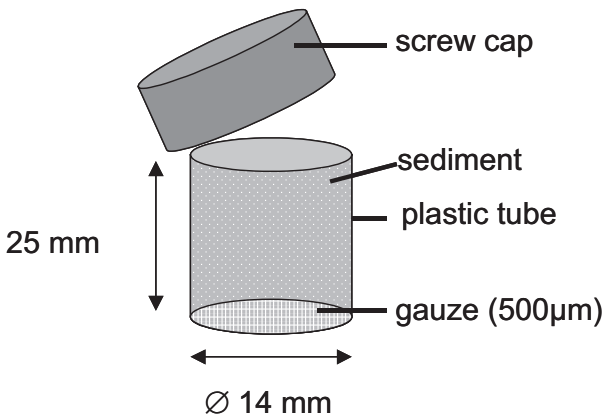
Fig. 1. Sediment cap (cylindrical plastic tubes) provided with a screw cap for closing in situ .
