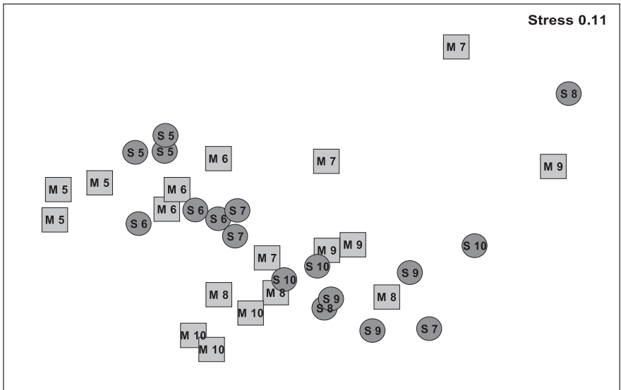
Fig. 3. Similarities (%) in taxonomic composition between algal communities of different months on mud (M) and on sand (S) in the Schöhsee sampled from May (M5, S5) to October (M10, S10) resulting from MDS ordination analysis. Absolute cell numbers in the top 500 \mu\text{m} of the sediments are considered.
