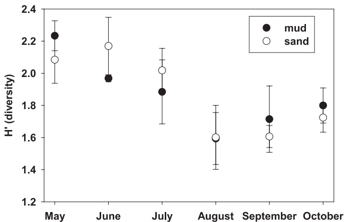
Fig. 5. Diversity ( H' ) of the algal community on mud and on sand in the Schöhsee sampled from May to October 2001. Mean values and error bars as standard deviations (SD) are given.
