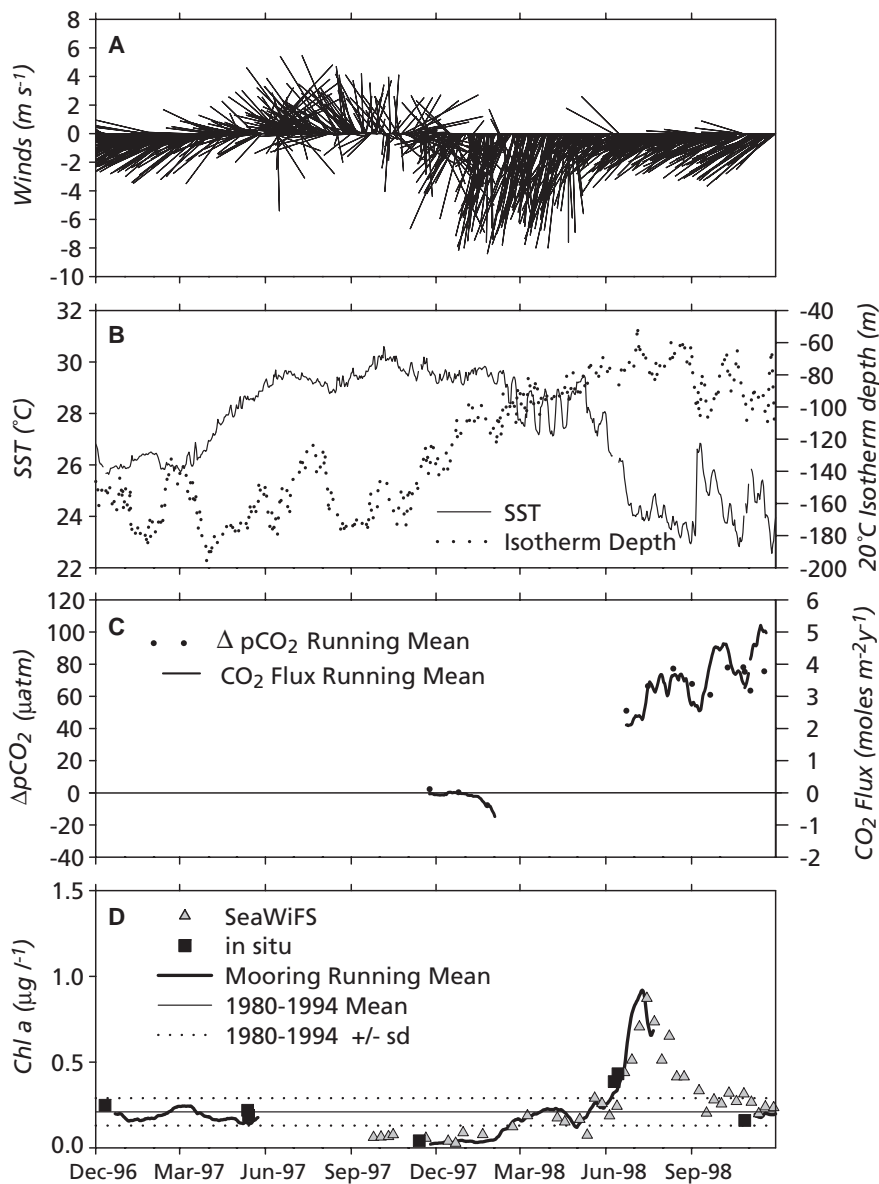
Figure 4: Wind speed and direction, sea-surface temperature and 20°C isotherm depth, \Delta p\text{CO}_2 values and \text{CO}_2 flux, and chlorophyll measured by instruments on a mooring at 0°, 155°W from December 1996 to December 1998. Chlorophyll measured on shipboard and from the SeaWiFS satellite are also plotted in panel D. Strong eastward currents associated with the movement of the warm pool caused the mooring to be pulled under and the instruments to fail in February 1998. The problem was corrected in June 1998.
