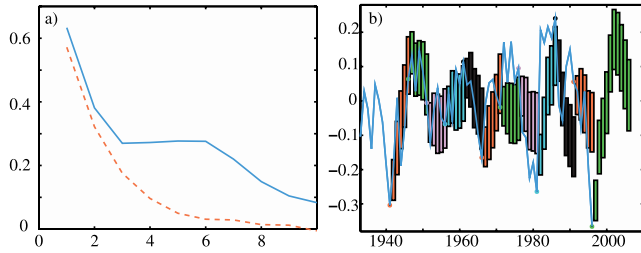
Figure 3. (a) Estimated correlation skill score for T_o of the AR5 model (solid blue line) and the AR1 model (dashed line) using all possible initial conditions for T_o . (b) Forecasts with the AR5 model compared to the “observed” T_o (solid blue line). The latter was obtained by projecting the detrended SST anomalies from the GISST [Rayner et al. , 1996] dataset on to the SST (feedback) pattern used to compute T_o in the model. The starting year of each ensemble of forecasts (5000 members) is denoted with a dot in different color coding. The figure shows bars for the bounds of the annual mean T_o in which 50% of the ensemble members are located. Each member of a particular ensemble of forecasts shares the previous 5 years of the observed T_o as initial condition, they differ from each other afterwards by the weather noise ( N ) only.
