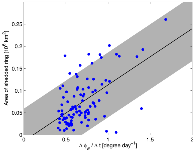
Fig. 10. The change in front location for loop occlusion events for the AVISO altimetry data (when \Delta\phi_w/\Delta t > 0.4 degree day ^{-1} ) versus the area of the associated ring being shed. The gray area denotes the 90% confidence band. The correlation coefficient of the data set is 0.59. Although the spread in data points is smaller than in the AG01 model (Fig. 4, note the different scales of the axes), both the linear relation and the width of the 90% confidence band are similar.
