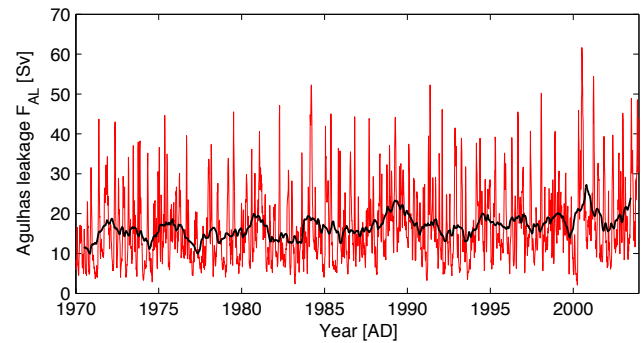
Fig. 6. Time series of the Agulhas leakage transport F_{AL} , the flux of water sampled by the numerical floats over the GoodHope line in red, and the one year smoothed time series in black. The mean magnitude of Agulhas leakage is 16.7 Sv, with a standard deviation of 9.2 Sv. The Agulhas leakage transport never gets to zero on this five day resolution.
