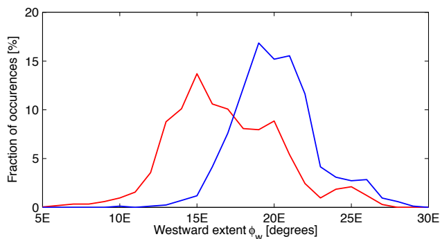
Fig. 12. Distributions of the non-smoothed westward extent of the Agulhas Current retroflection \phi_w for the AGO1 model data (red line) and the AVISO altimetry data (blue line). For high values of the westward extent (early retroflections, \phi_w > 23^\circ E) the distributions of the two data sets are similar, but the low \phi_w tail in the model data is much more westward than for the altimetry data. This explains the relatively low variability in AVISO E_{AL} compared to the variability in AGO1 data (Fig. 11). The wider distribution, especially on the low \phi_w tail, of the model data is also related to the larger rings that are shed in the model (compare Fig. 4 with Fig. 10).
